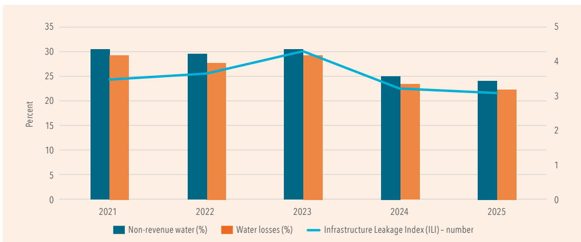
Figure 23: Trends in non-revenue water (%), water losses (%) and the Infrastructure Leakage Index (ILI), indicating improved network efficiency and leak management
