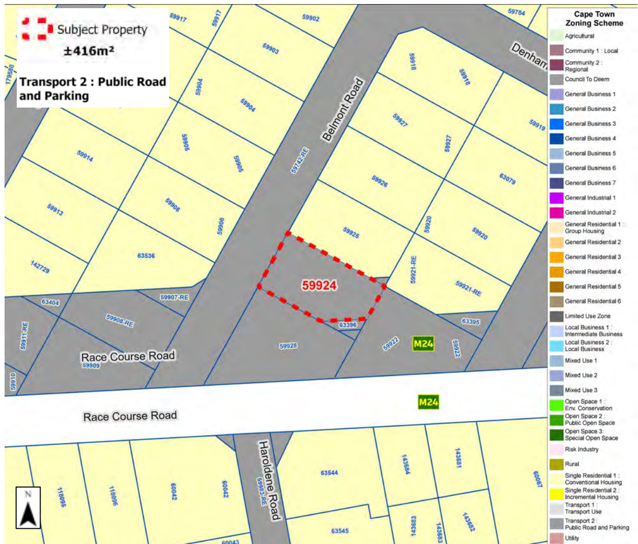
Figure 4: Proposed Rezoning
