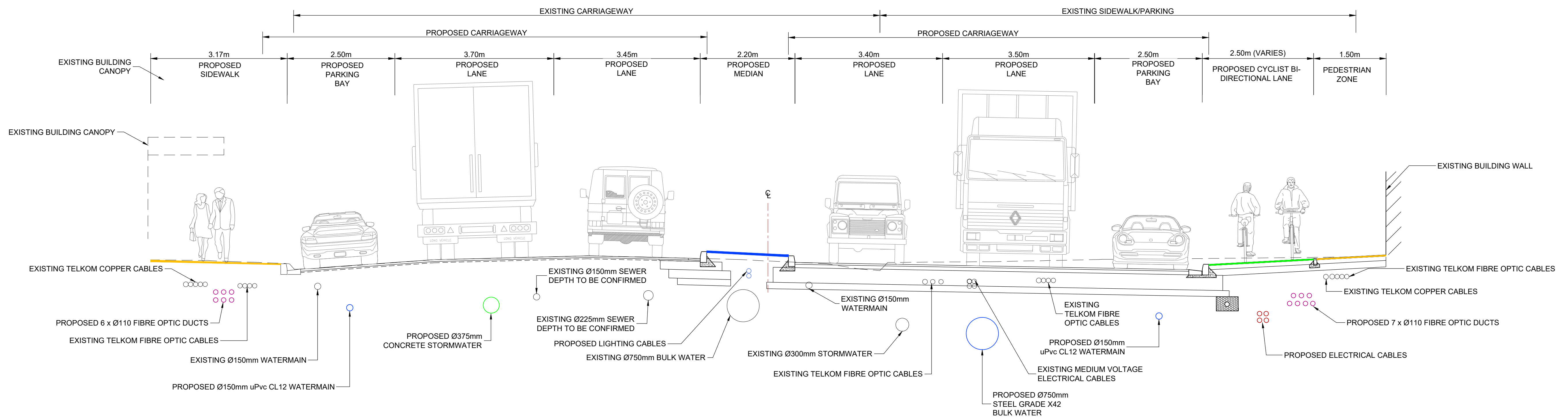
SV1650 TYPICAL SECTION D-D SCALE 1:50
